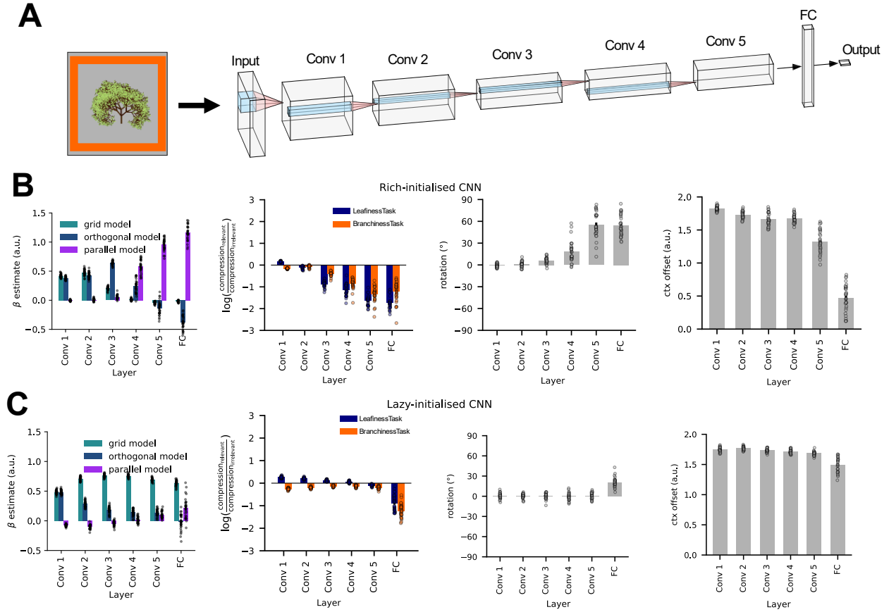
Fig. S6. Convolutional Neural Network (CNN) trained on the same stimuli as human participants.
